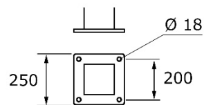
Flange with 4 holes \varnothing 18 mm (option)
