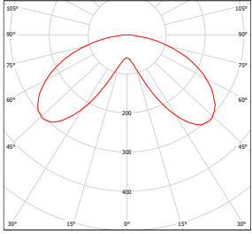
BALK30C2
