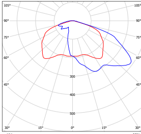
BALK20T4, BALK30T4
