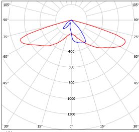
BALK20, BALK30
